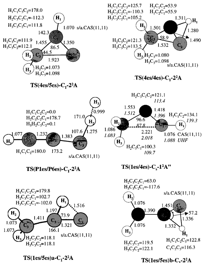
Figure 5. CASSCF(11,11)/6-311+G(d,p) optimized geometry of the transition states of the C(^3P) + C_2H_3 reaction on the first excited-state PES. Bond lengths are in Å and bond angles are in degrees. Symmetry of the species and their electronic states are also specified.
