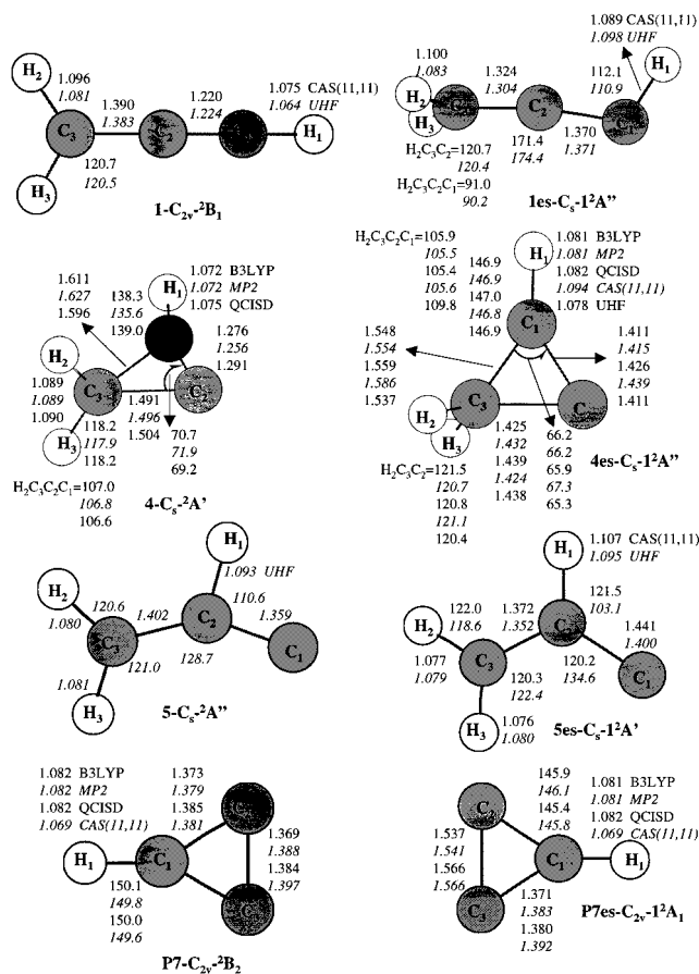
Figure 4. CASSCF(11,11)/6-311+G(d,p) optimized geometry of the local minima of C_3H_3 and c-C_3H species on the first excited-state PES. Bond lengths are in Å and bond angles are in degrees. Symmetry of the species and their electronic states are also specified.
